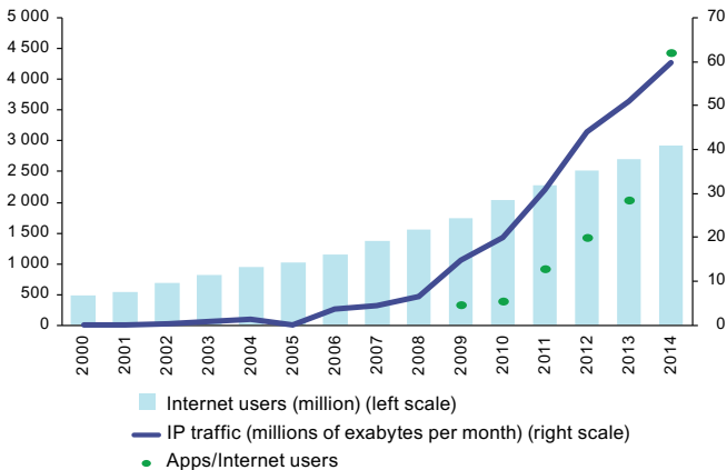
■ Figure I.5 ■ Global growth of IP traffic, number of Internet users and applications downloaded, 2000-2014
